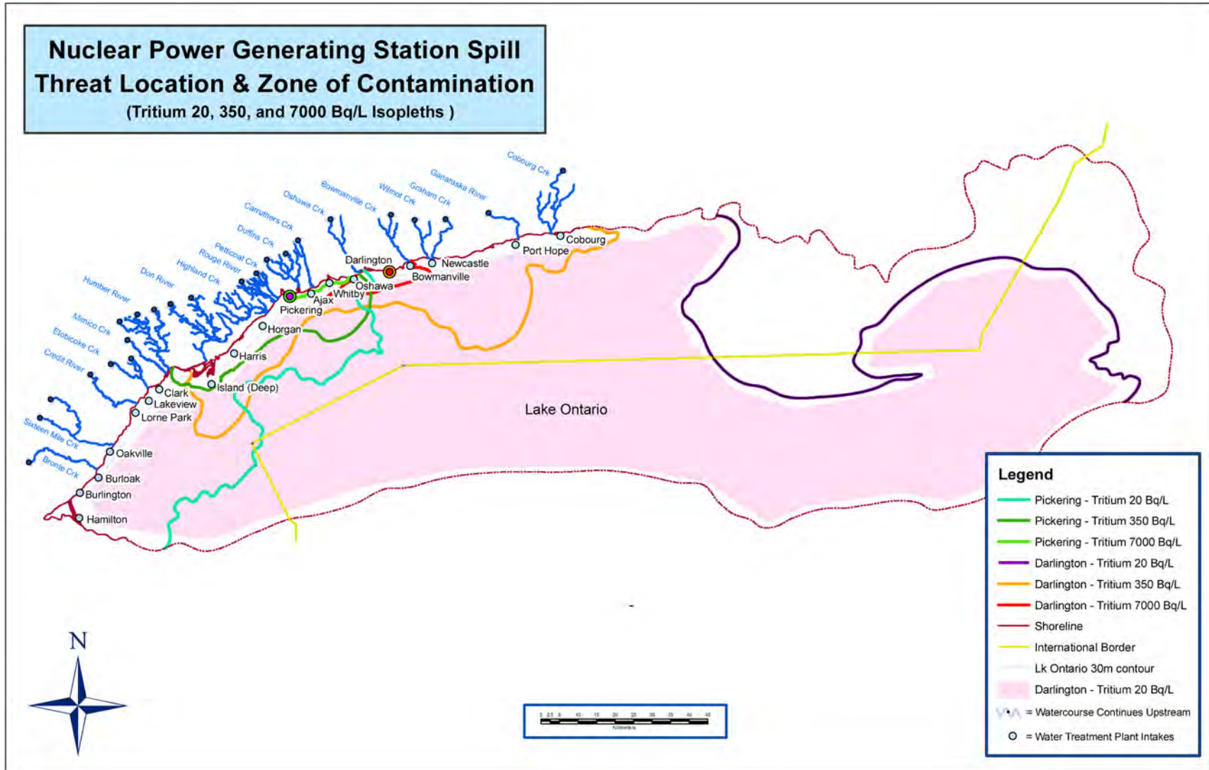
Figure E6-37: Nuclear Power Generating Station Spill Threat Location and Zone of Contamination (Tritium 20, 350 and 7000 Bq/L Isopleths)
