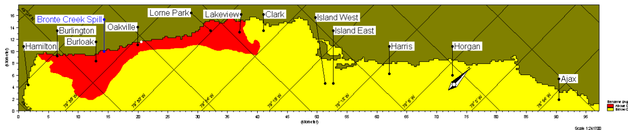
Figure E6-24: Oakville Storage Facility Spill - 0.05 mg/L Benzene Isopleth
