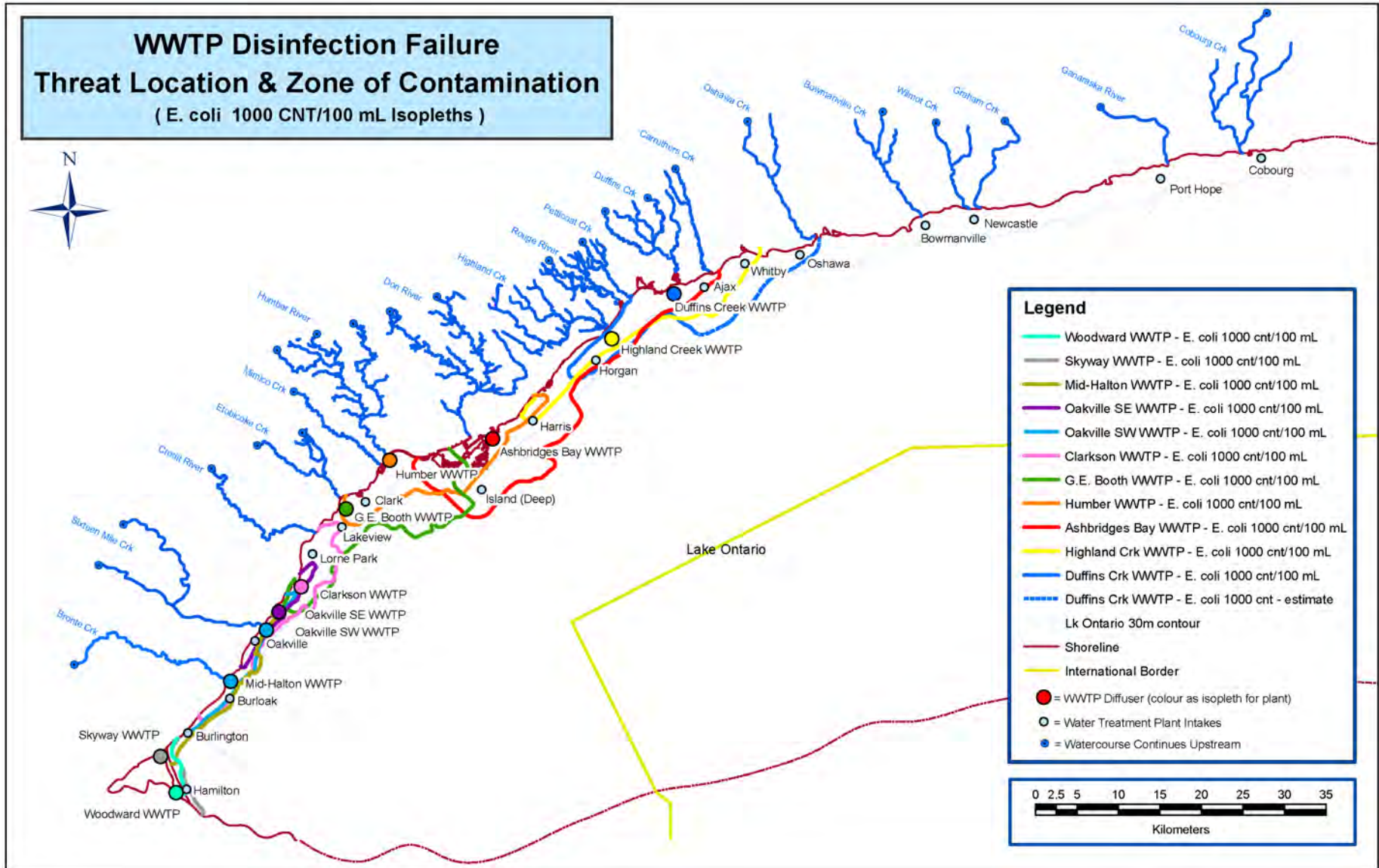
Figure E6-33: WWTP Disinfection Failure Threat Location and Zone of Contamination ( E. coli 1000 CFU/100 ml Isopleths)
