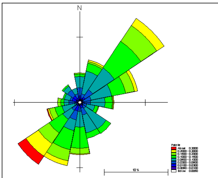
Figure E6-7: Calculated Current Compass Rose in Pickering section of Coastal Zone
