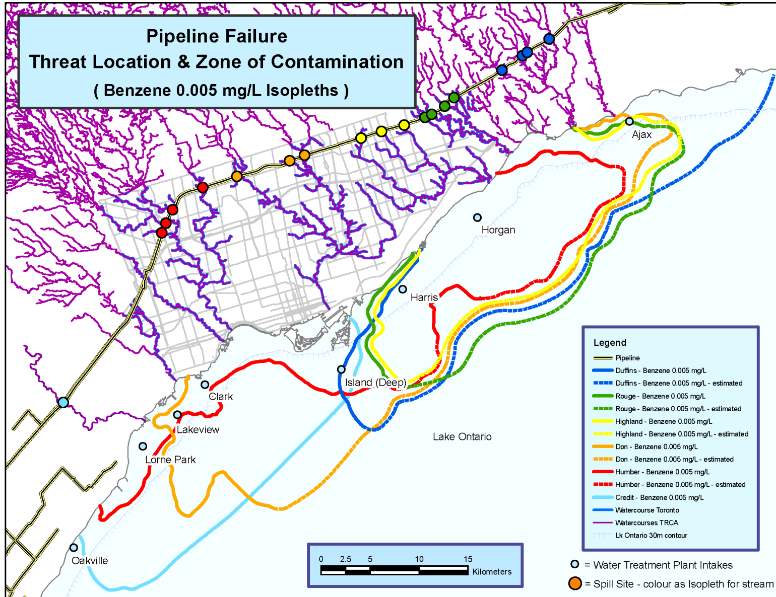
Figure E6-36: Pipeline Failure Threat Location and Zone of Contamination (Benzene 0.005 mg/L Isopleths)
