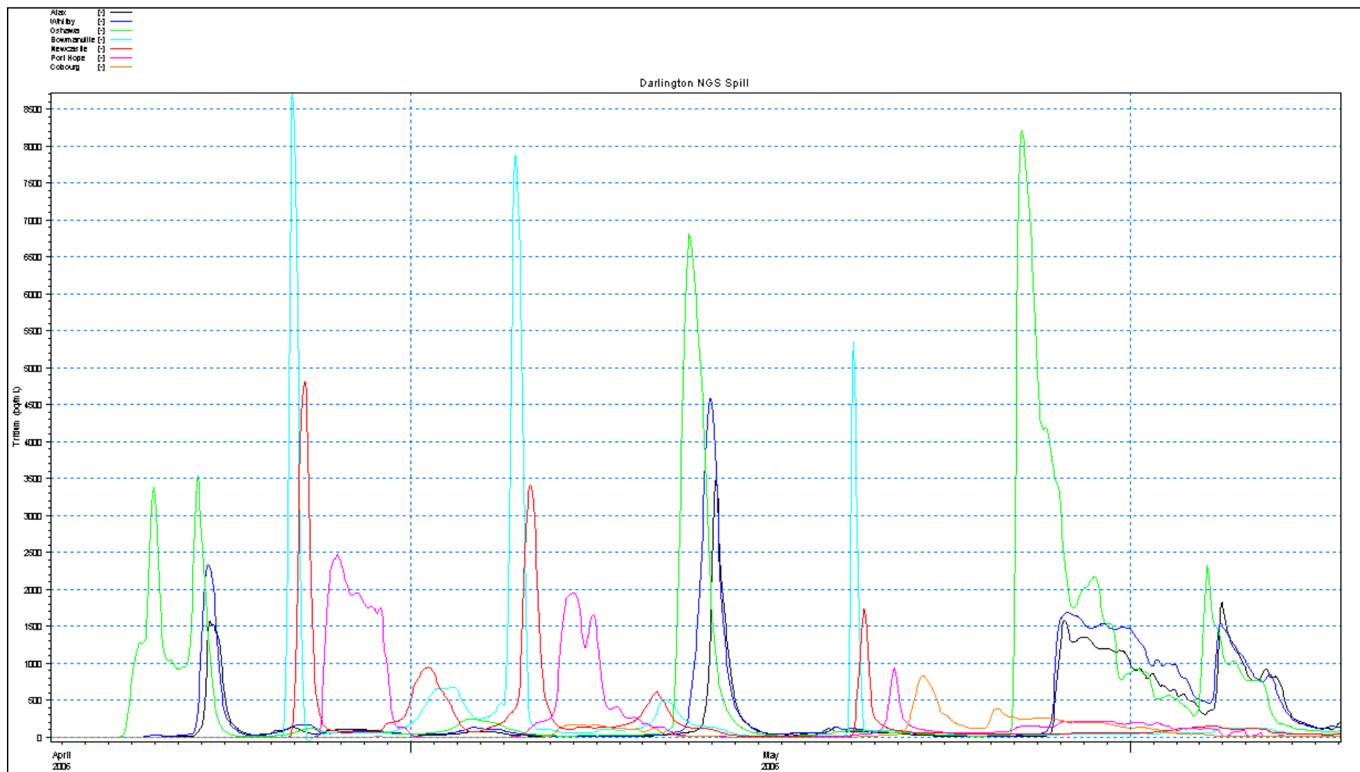
Figure E6-27: Tritium time series at Intakes (Ajax to Cobourg) for release from Darlington outfall
