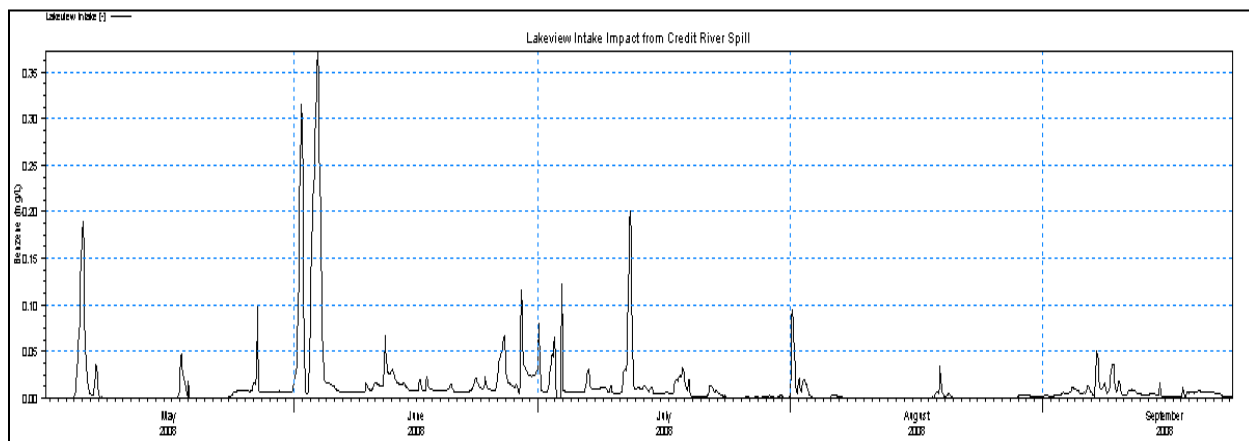
Figure E6-21: Lakeview (now Arthur P. Kennedy) time series from Credit River
