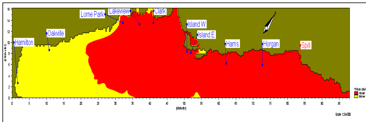
Figure E6-28: Extent of Contamination for Tritium, using a 150 Bq/L contour.
