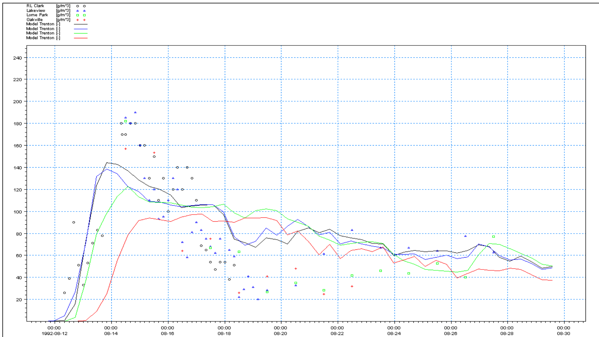
Figure E6-26: Model Calibration: Comparison of Model Calculations with observations using Trenton Winds for Clark to Oakville intakes
