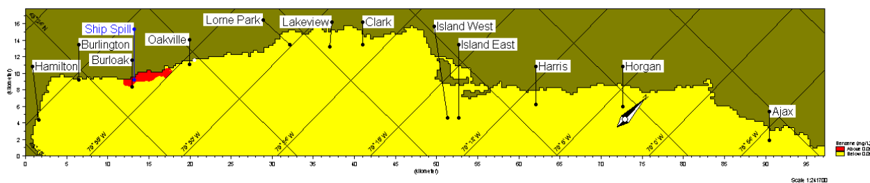
Figure E6- 25: Scenario of 1000 L spill with a Benzene Isopleth of 0.05 mg/L
