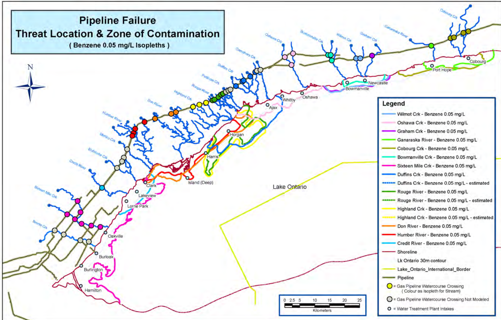
Figure E6-35: Pipeline Failure Threat Location and Zone of Contamination (Benzene 0.05 mg/L Isopleths)
