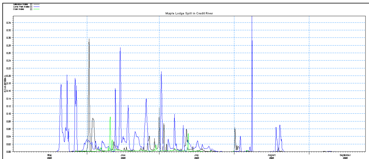
Figure E6-20: Predicted E. coli Densities from Industrial Animal Food Processing Lagoon Scenario
