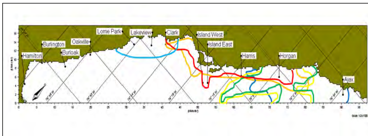
Figure E6-22: Composite Contaminant Map for Benzene from Pipeline Spill at GTA Watercourse Crossings
