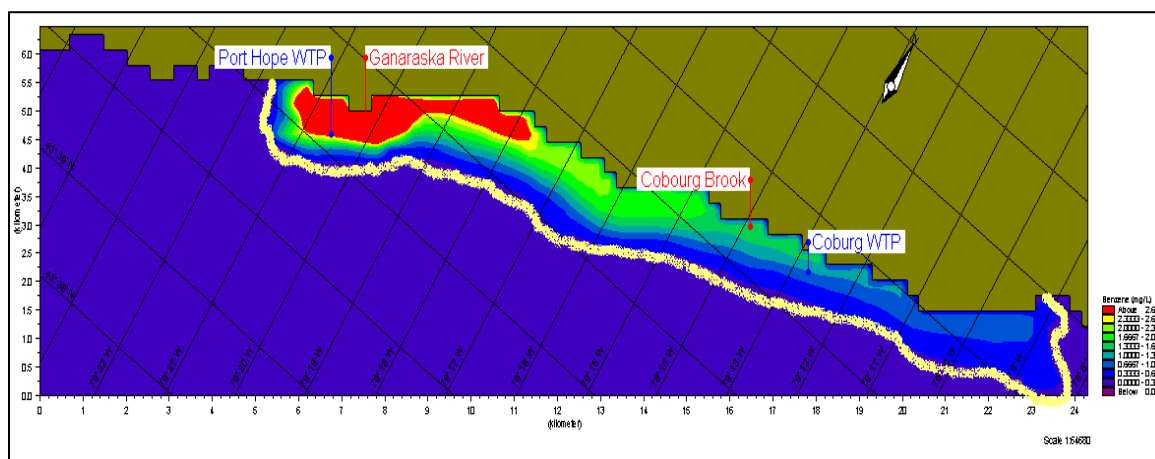
Figure E6-29: Boundary for Benzene Spill for Ganaraska River – Easterly Plume.
