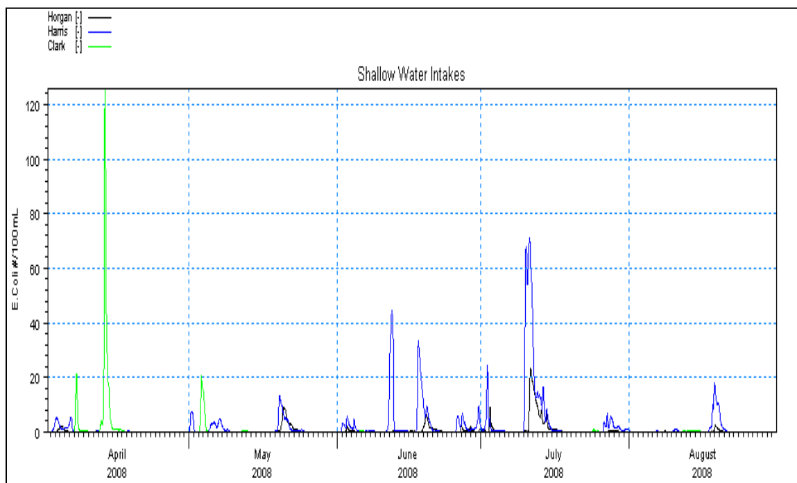
Figure E6-18: E. coli Levels for Horgan, Harris, and Clark from CSO spill
