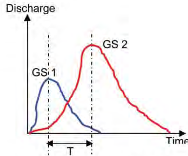
Fig.2: Illustration of unit hydrographs related to time of travel (ToT).
