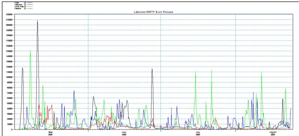
Figure E6-16: Composite Contaminant Map for E. coli from Disinfection Failures at GTA area WWTP's.
