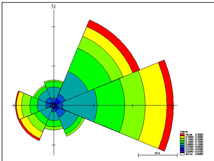
Figure E6- 6: Calculated Current Compass Rose in Etobicoke section of Coastal Zone
