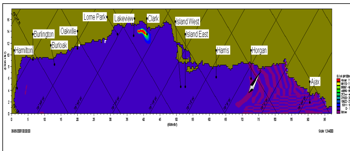
Figure E6-31: Spatial Extent of Impact from Spill occurring Aug 5.
