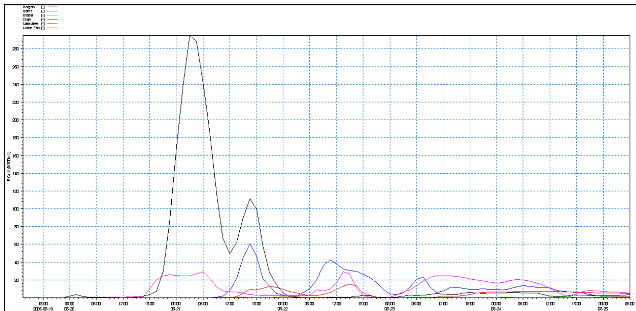
Figure E6-17: E. coli time series for STS Breaks
