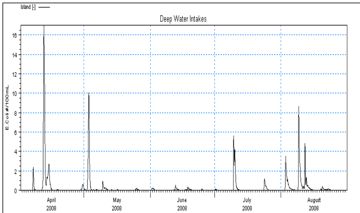
Figure E6-19: E. coli Levels Predicted for Toronto Island intakes from CSO spill
