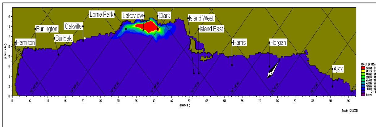
Figure E6-32: Spatial Extent of Impact from Spills starting April 4 for a Four-week period.
