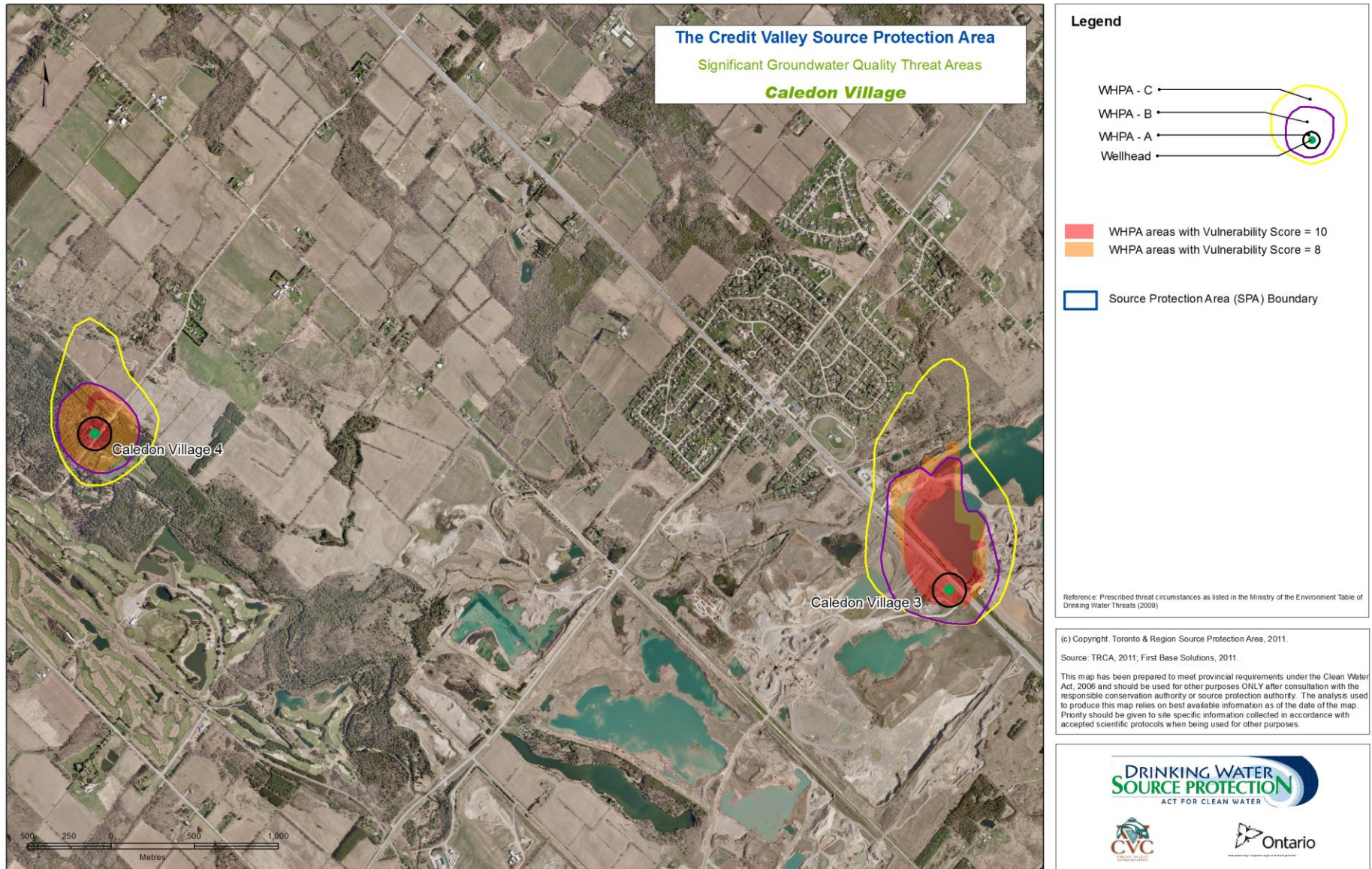
Map 1.8: Caledon Village – Significant Groundwater Quality Threat Areas
