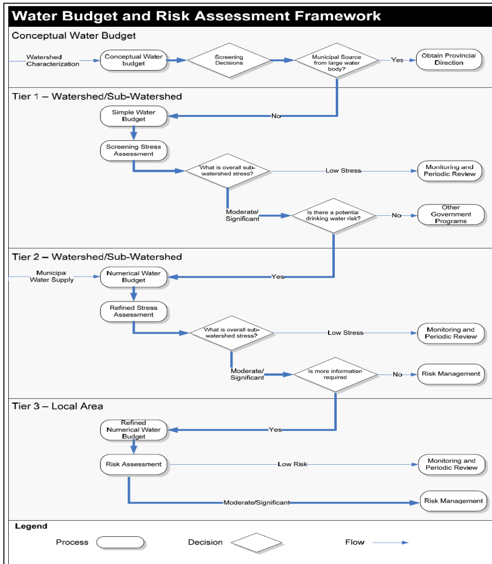
Figure C1. 1: Illustrates the Water Budget Framework (Technical Rules)
