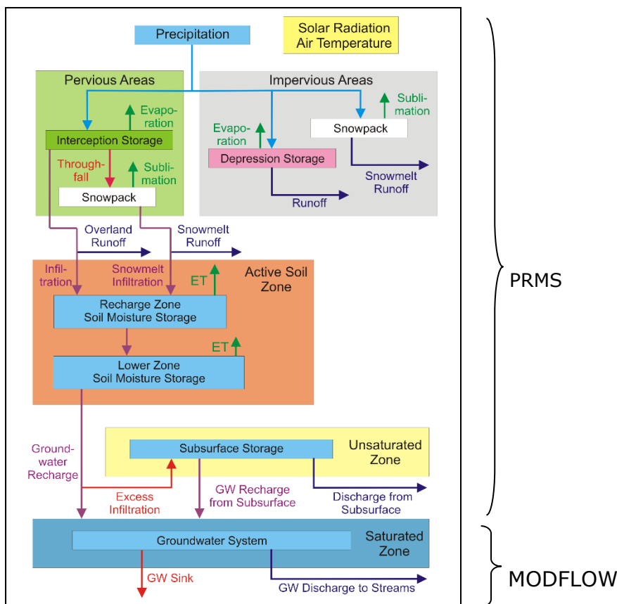
Figure C2. 1: PRMS/MODFLOW model process integration (EarthFx, 2007)
